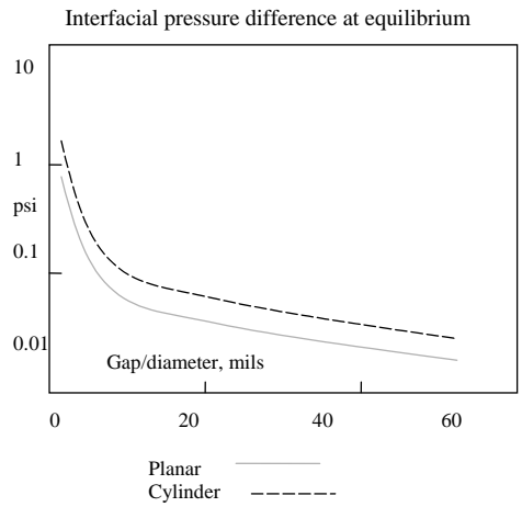
Figure 2: Relationship between gap size and capillary force for water on glass
